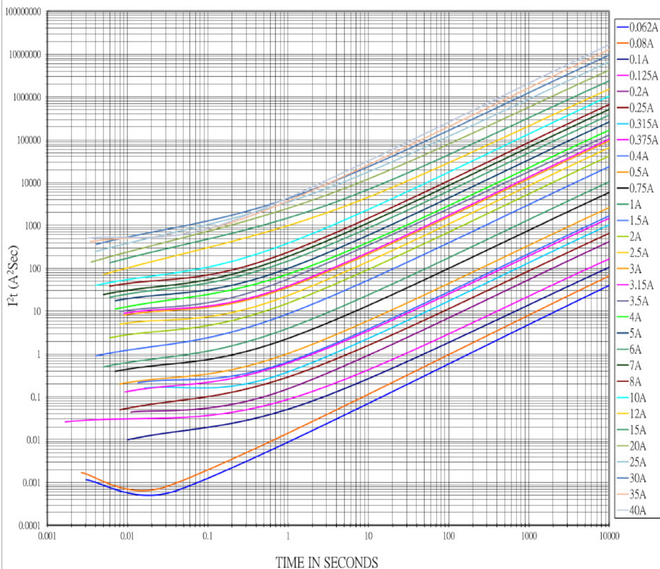
Average Melting I^2t Curves
